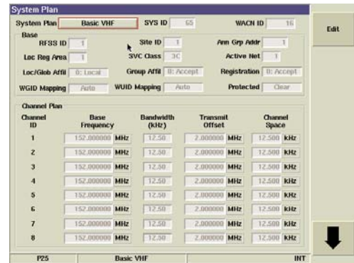
P25 Trunking Configuration
